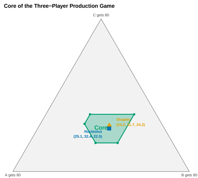
Figure 12.1: The core of the three-player production game (shaded polygon) within the efficiency simplex. The Shapley value (triangle) and nucleolus (square) both lie inside the core, confirming both solution concepts yield stable allocations.
