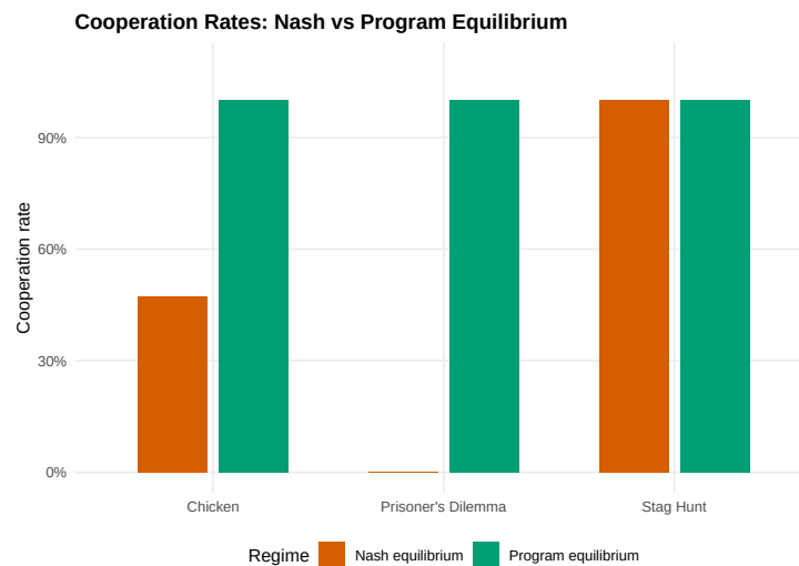
Figure 41.1: Cooperation rates (fraction of agents playing the cooperative action) under Nash equilibrium vs program equilibrium across three classic games. Commitment enables full cooperation in all games, including the Prisoner's Dilemma where Nash equilibrium yields zero cooperation.
