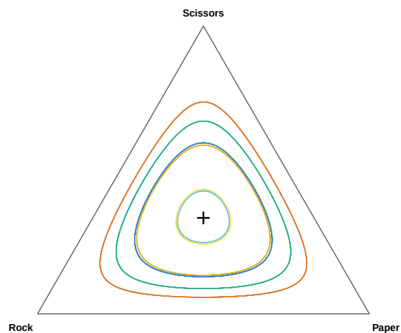
Figure 20.1: Replicator dynamics for Rock-Paper-Scissors on the two-dimensional simplex. Six trajectories from random initial conditions cycle around the interior equilibrium at (1/3, 1/3, 1/3) . The orbits are closed curves — the system never converges, reflecting the non-transitive dominance structure of the game.
