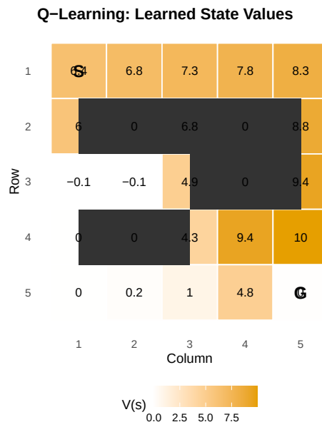
Figure 25.1: Learned state values (max Q per state) in the 5x5 gridworld. The agent starts at (1,1) and must reach the goal at (5,5). Dark cells are obstacles. Higher values (orange) indicate states closer to the goal along the optimal path.
