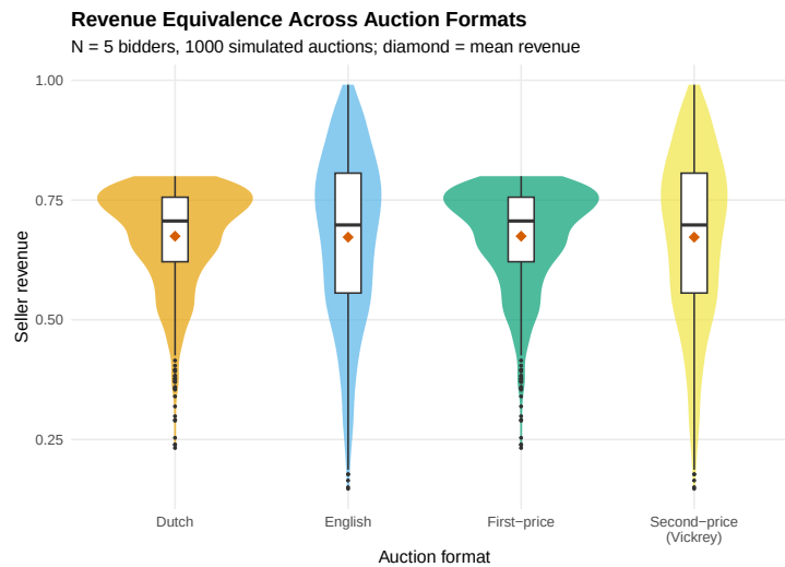
Figure 32.1: Expected revenue comparison across four auction formats with 5 bidders and 1000 simulated auctions. Revenue equivalence holds: all formats yield similar expected revenue.
