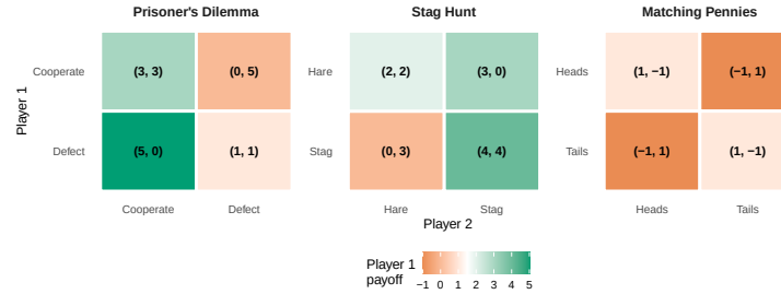
Figure 2.1: Payoff matrices for three canonical 2x2 games. Cell colour encodes Player 1's payoff using a diverging Okabe-Ito-inspired palette; each cell displays both players' payoffs as an ordered pair.
