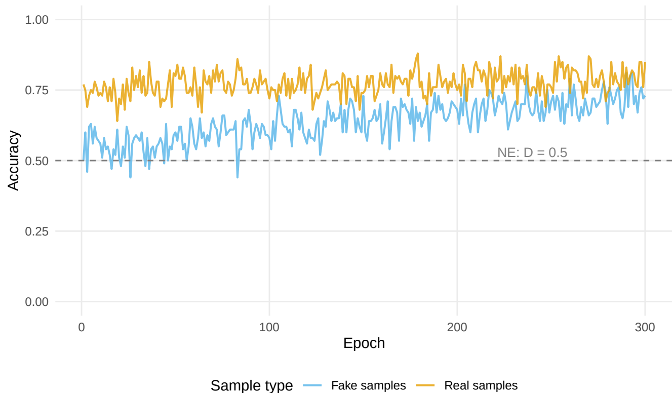
Discriminator Accuracy Over Training
