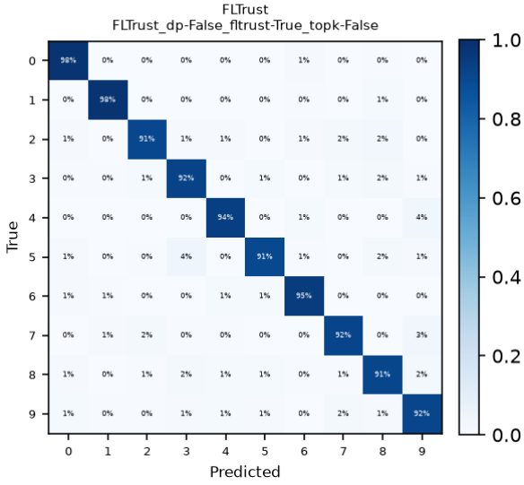
Figure 4: Final confusion matrices for FLTrust config.
