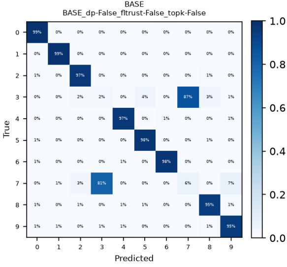
Figure 3: Final confusion matrices for standard FedAvg .
