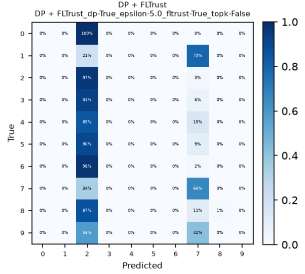
Figure 5: Final confusion matrix for the DP+FLTrust configuration.
