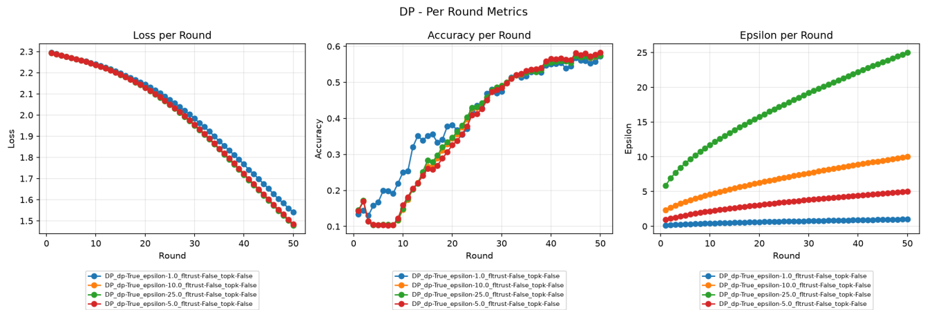
Figure 7: Accuracy per training round for DP-only configuration.
