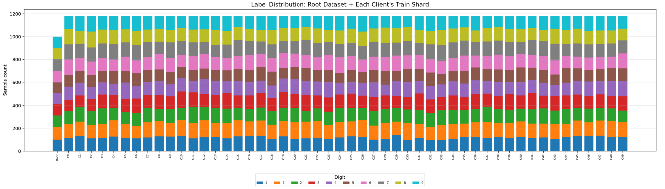
Figure 9: Label distribution of the root dataset used for FLTrust and the client training datasets. The root dataset was sampled uniformly across all classes, while the client datasets were sampled randomly.
