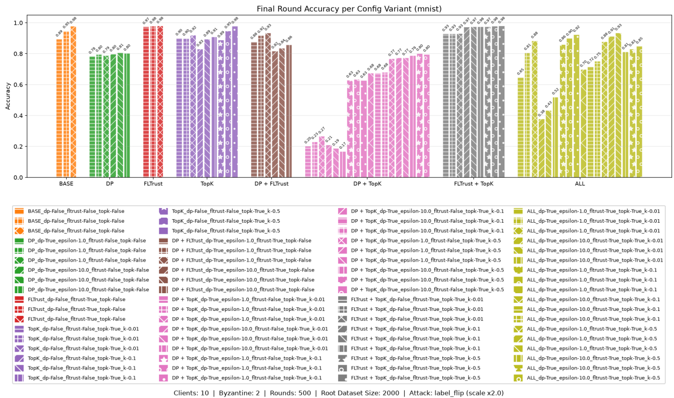
Figure 13: Final accuracy achieved on all different configurations.
