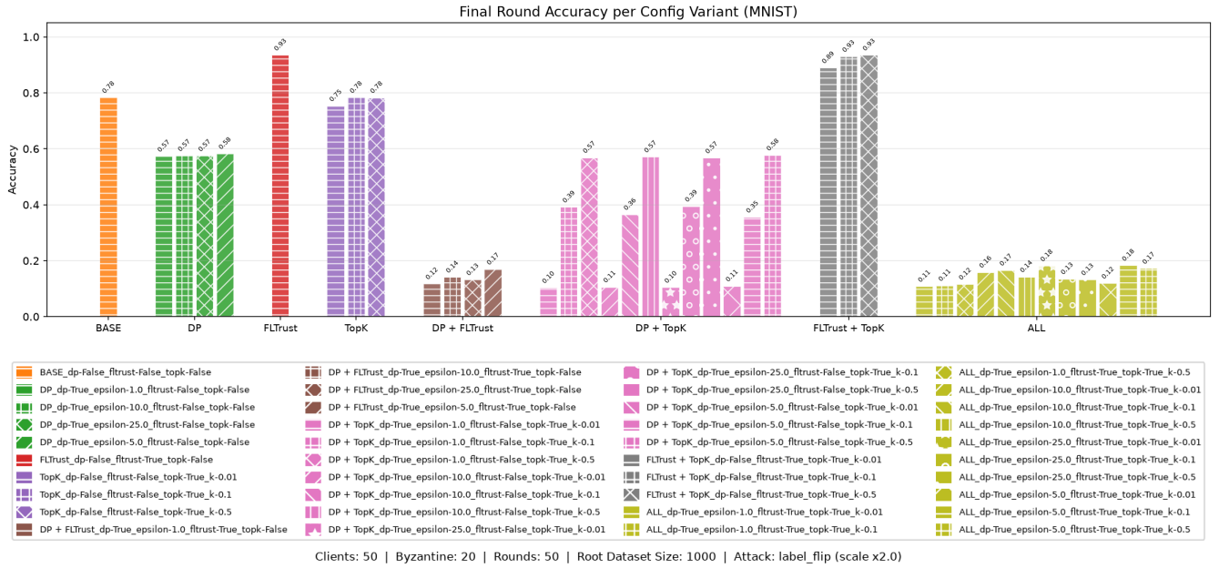
Figure 10: Final accuracy achieved on all different configurations.
