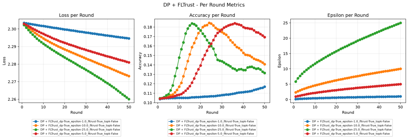
Figure 12: Accuracy per training round for DP+FLTrust configuration.
