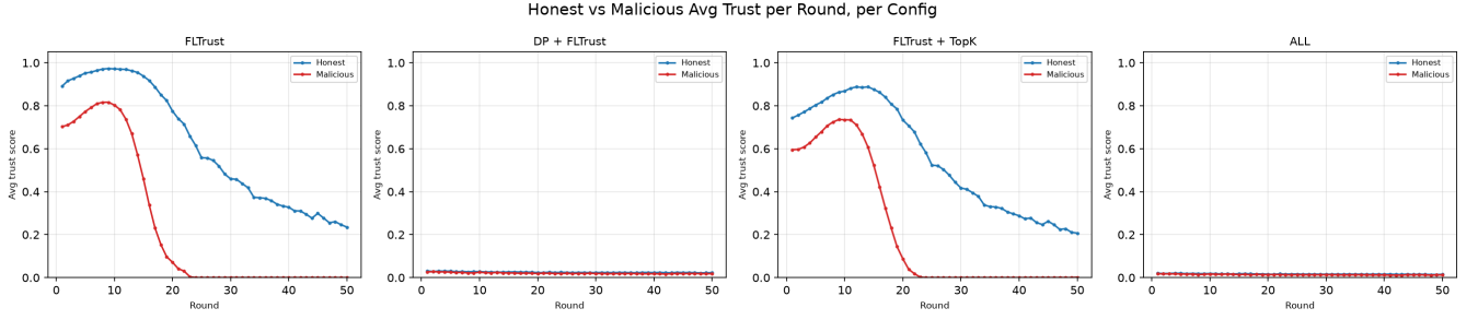
Figure 5: The line charts depict the average trust scores of honest and malicious clients during 50 rounds of full epochs trained, n = 50 , \eta = 0.4 , attack scale = 2.0. While for settings where DP is enabled the scores are consistently equally low, the settings without DP-related noise addition show a clear distinction.
