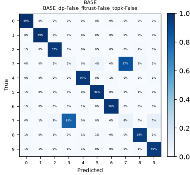
Figure 6: Final confusion matrices for standard FedAvg .
