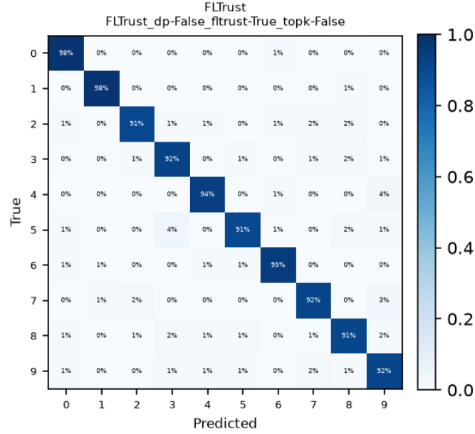
Figure 7: Final confusion matrices for FLTrust config.
