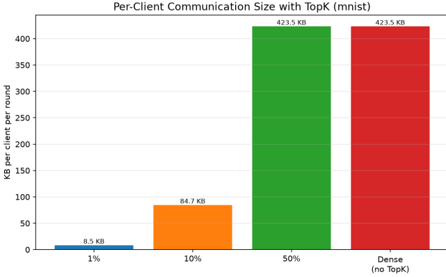
Figure 4: KB transferred per client per round for settings with different Top- k sparsification thresholds.
