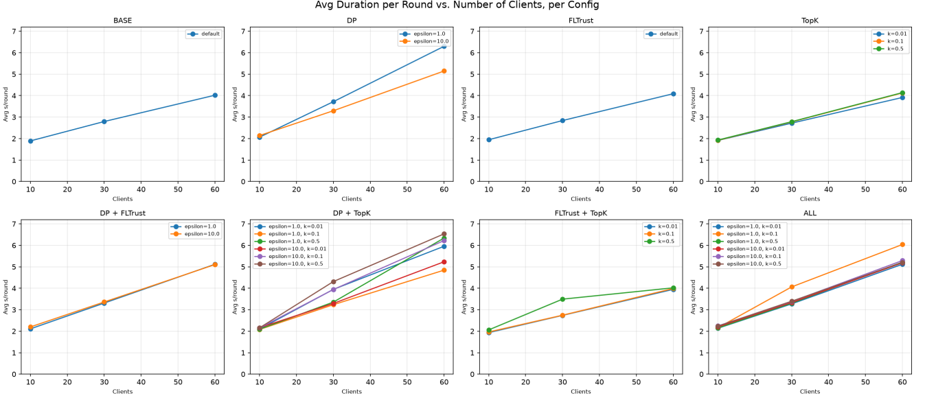
Figure 3: The average training duration per round for varying numbers of clients. Training run on MNIST dataset with 500 rounds of 10 SGD steps each, n \in \{10, 30, 60\} , \eta = 0.2 , attack scale = 2.0
