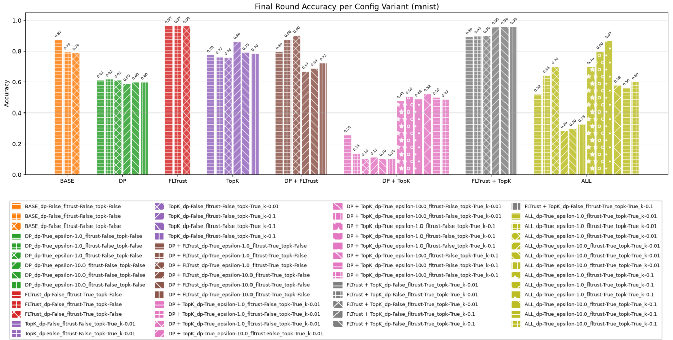
Figure 14: Final accuracy achieved on all different configurations.
