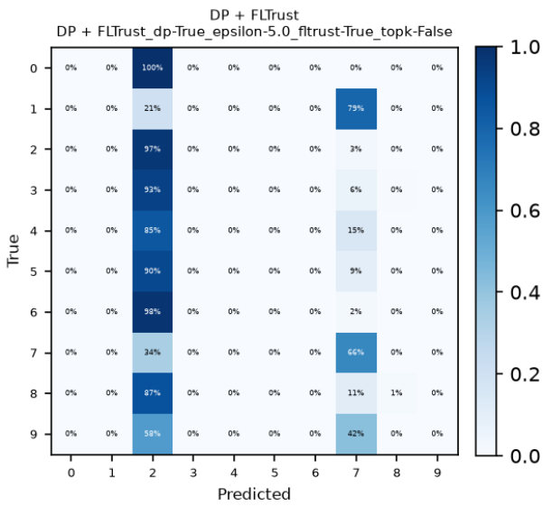
Figure 10: Final confusion matrix for the DP+FLTrust configuration.
