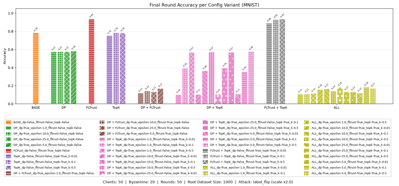
Figure 12: Final accuracy achieved on all different configurations.
