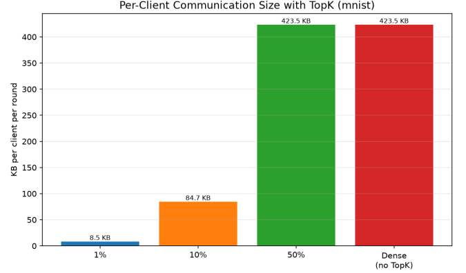
Figure 5: KB transferred per client per round for settings with different Top- k sparsification thresholds.
