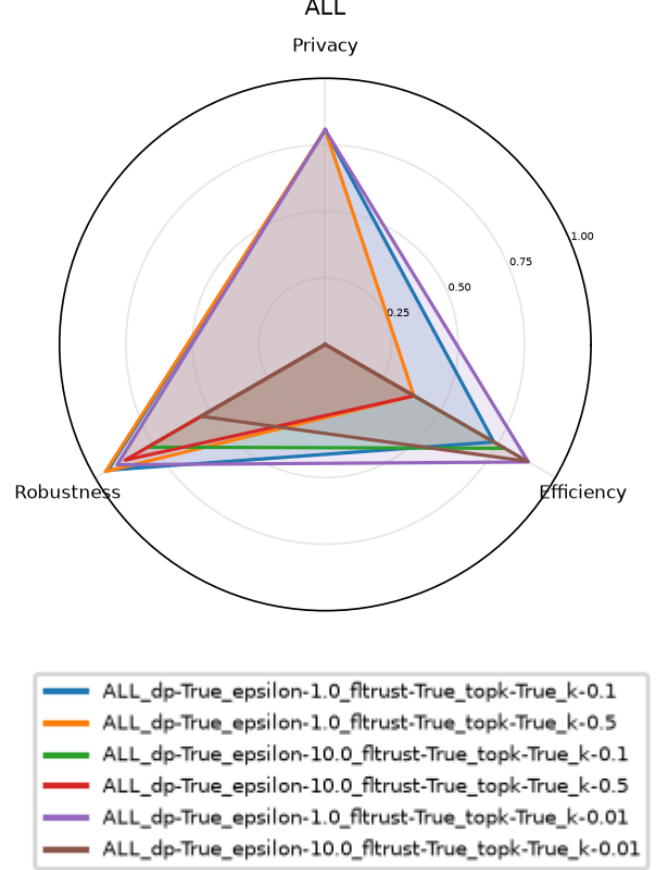
Figure 2: This chart depicts the results for the experiments on MNIST dataset with 500 rounds of 10 local (SGD) steps each, n = 60 , \eta = 0.2 , attack scale = 2.0
