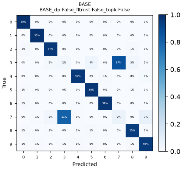
Figure 8: Final confusion matrices for standard Fe-dAvg .
