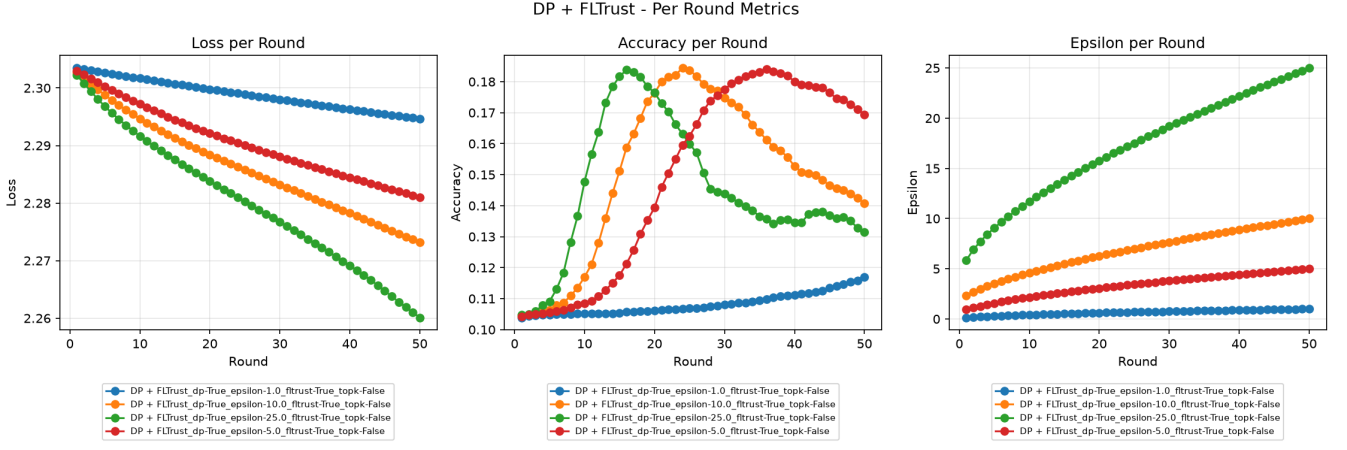
Figure 14: Accuracy per training round for DP+FLTrust configuration.
