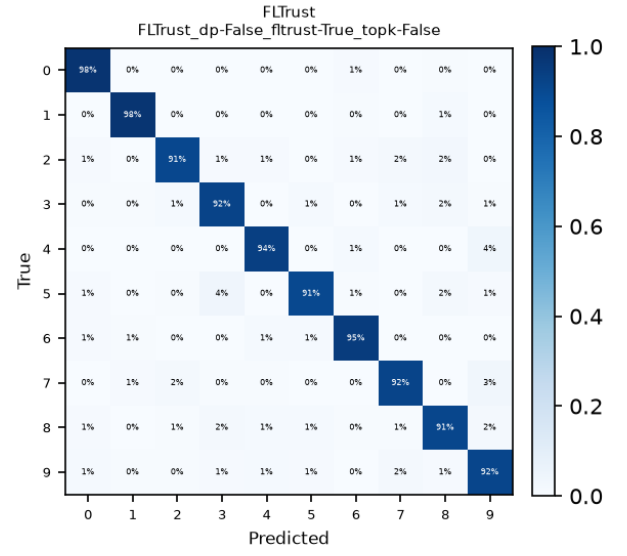
Figure 9: Final confusion matrices for FLTrust config.
