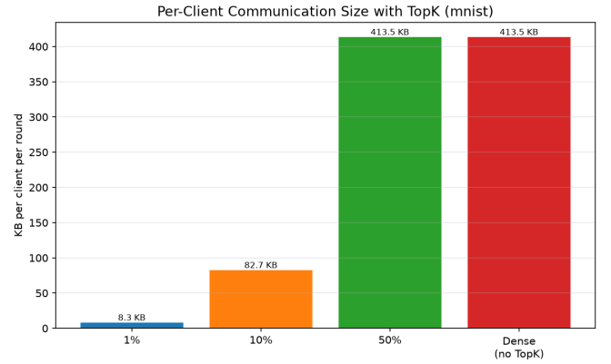
Figure 3: Bytes transferred per client per round for settings with different Top-k sparsification thresholds.
