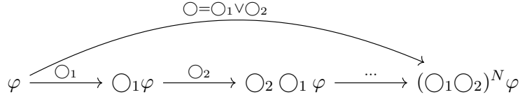
FIGURE 1. The join as the limit of alternating iterates: finite on a finite poset ( N = |P| , Theorem 4.1), transfinite in general, and not a \mathbf{PLL}_2 -formula (Theorem 5.1).
