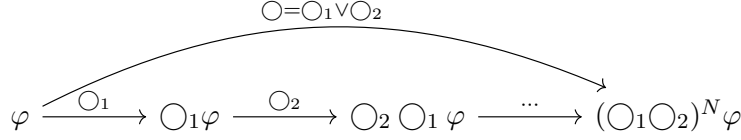
FIGURE 1. The join as the limit of alternating iterates: finite on a finite poset ( N = |P| , Theorem 4.1), transfinite in general, and not a PLL 2 -formula (Theorem 5.1).
