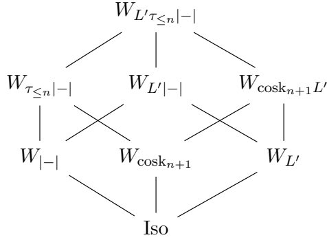
FIGURE 1. The sublattice of \text{Same}(\text{Fun}(\Delta^{\text{op}}, \mathcal{E})) generated by the three classes: every join is the class of equivalences of a reflector (Theorem 4.1, Proposition 5.1, Theorem 5.2). Lines are joins, read upwards; incomparabilities are not asserted.
