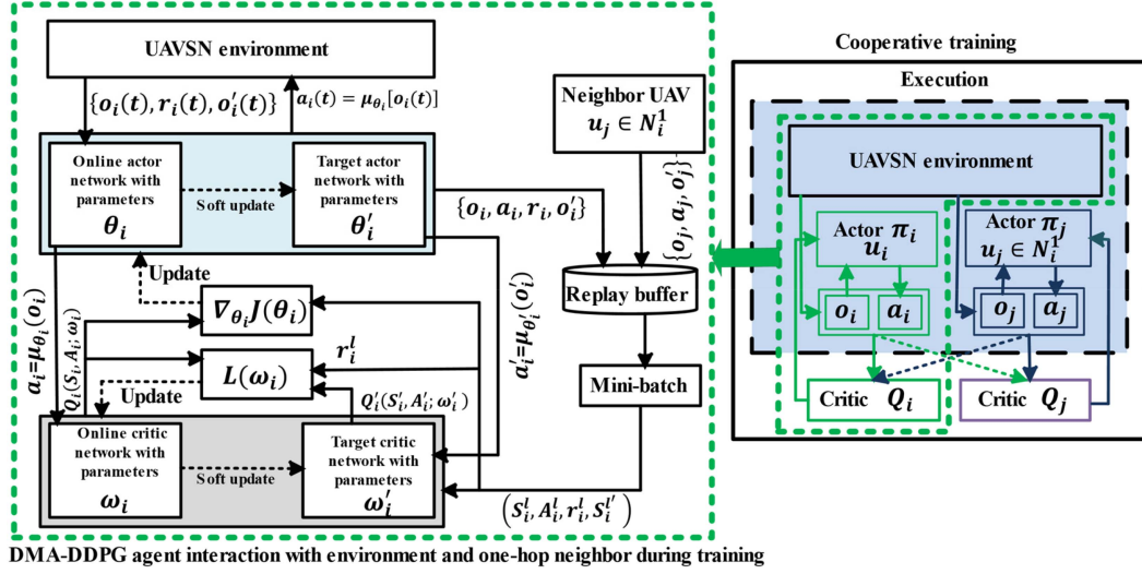
Fig. 3. Adaptive DMA-DDPG training process and neural network architecture of an agent UAV.
