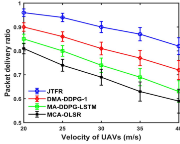
(a) Packet delivery ratio (PDR)
