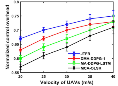
(c) Normalized control overhead (NCO)
