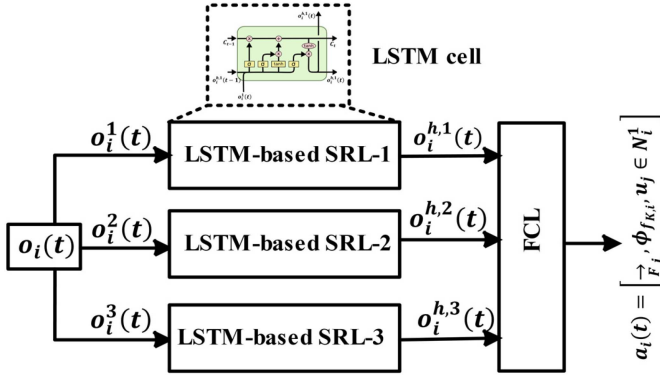
Fig. 4. Structure of an actor network.
