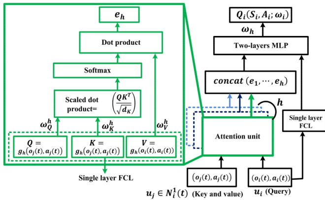
Fig. 5. Structure of a multi-head attentional critic network.
