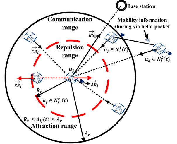
Fig. 2. Behavior-based motion model of UAVs in UAVSNs.
