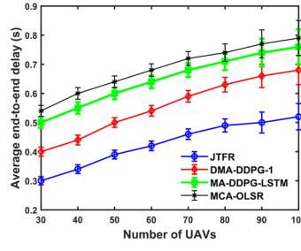
(b) Average end-to-end delay (AE2ED)
