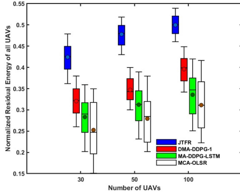
Fig. 10. Normalized residual energy (NRE).
