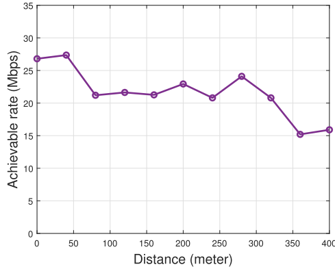
Fig. 8. Achievable rate between two UAVs.
