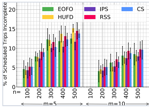
Fig. 7. % incomplete trips when using real-world drone energy traces. None of the trips fail for n \leq 80 .
