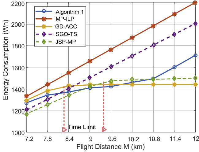
Fig. 3. The energy usage against the required delivery distances, when the specified delay T is 30 min.
