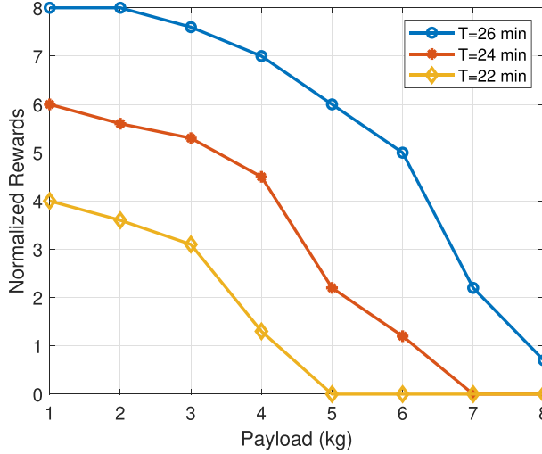
Fig. 10. The normalized in-situ sensing rewards under different payloads of the drone, as T increases.
