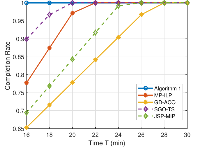
Fig. 5. The timely flight completion ratio of the flight distance M = 8.4 km, as the allowed flight time T increases.
