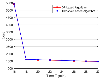
(a) Total cost with the increase of required arrival time T for M = 10.2 km
