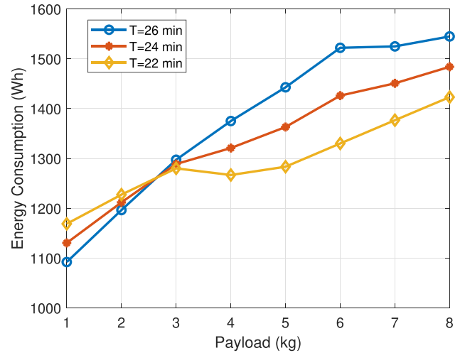
Fig. 9. Total energy consumption under different payloads of the drone, as T increases.
