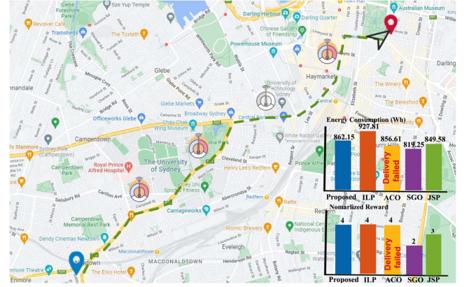
Fig. 11. The map of the on-campus case study: the required delivery distance M = 4.55 km when the specified delay T is 14 min.
