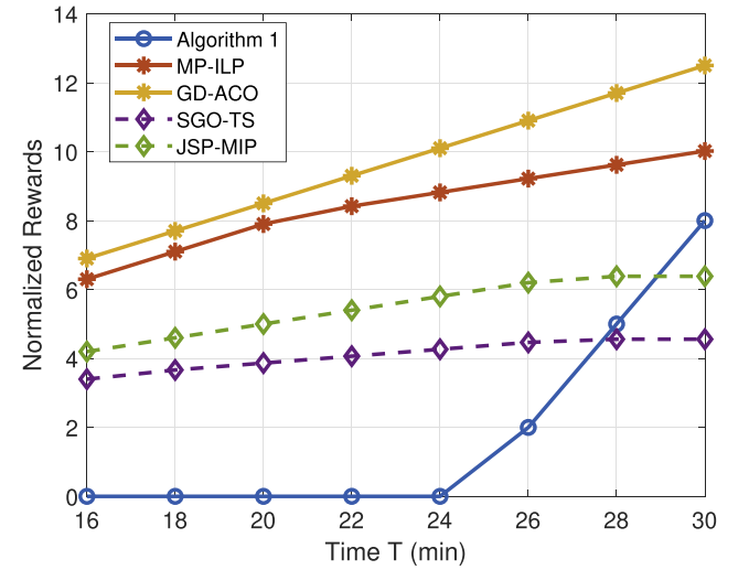
Fig. 6. The normalized in-situ sensing rewards for M = 8.4 km, as T increases.
