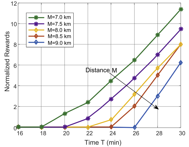
Fig. 8. The normalized in-situ sensing rewards under different flight distances, as the allowed flight time T increases.
