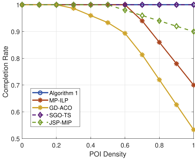
Fig. 7. The timely flight completion ratio under different POI densities \rho(\mathcal{L}^{(1)}) .
