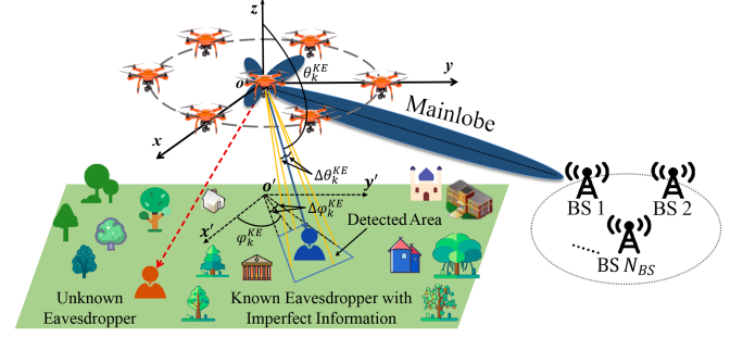
Fig. 1. A UAV-enabled secure communication system exploiting CB.
