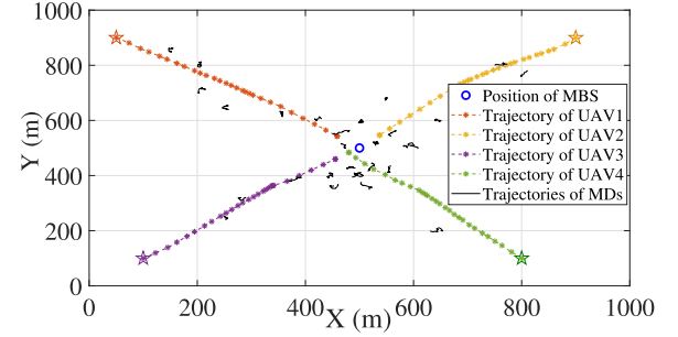
Fig. 4. Trajectories of the MDs and UAVs.
