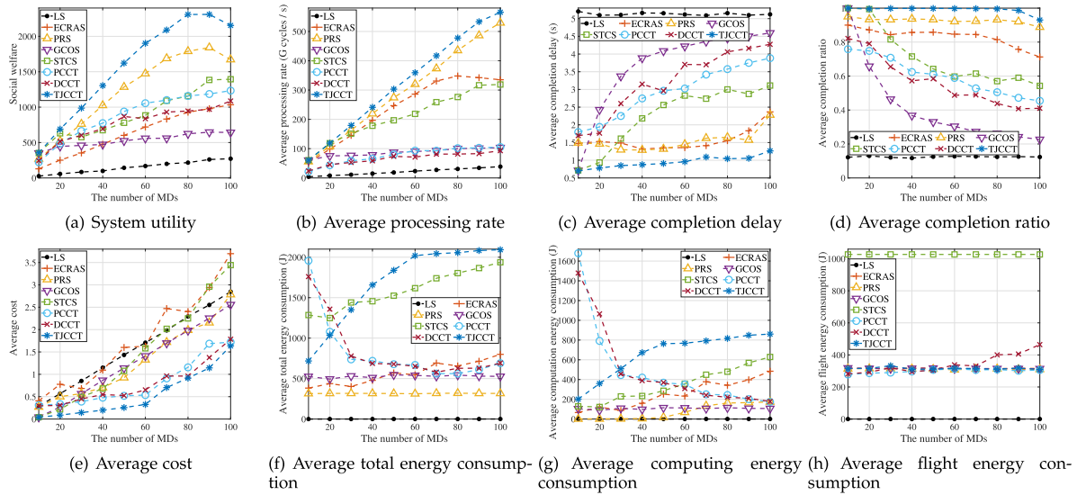
Fig. 3. System performance with the number of MDs.
