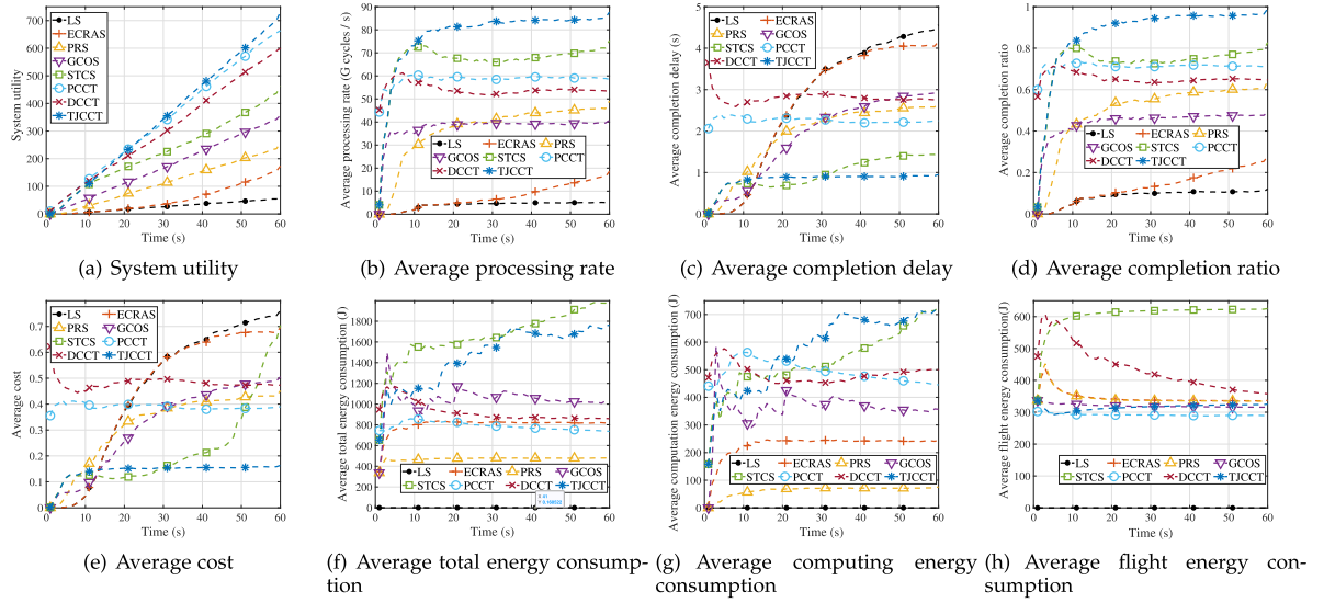
Fig. 2. System performance with time.
