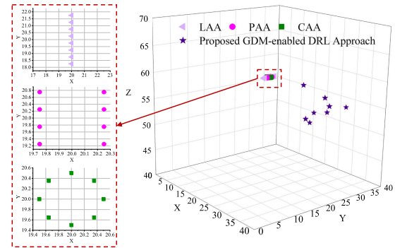
Fig. 5. Comparison of position distributions of UAVs in different deployment policies.
