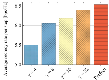
Fig. 11. Performance analysis under imperfect phase synchronization.
