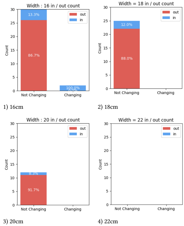
(b) Entry/Exit collision points across varying widths
