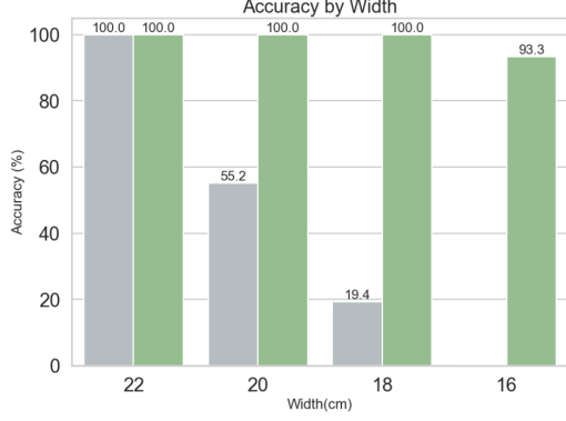
Figure 2. Experimental results of the sensitivity analysis varying hole entrance width. The Baseline fails significantly as width decreases.
