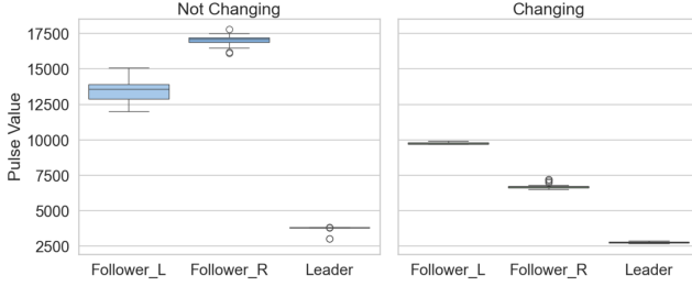
Figure 4. This figure shows the distance traveled measured using the encoder counters of the Leader and Follower.
