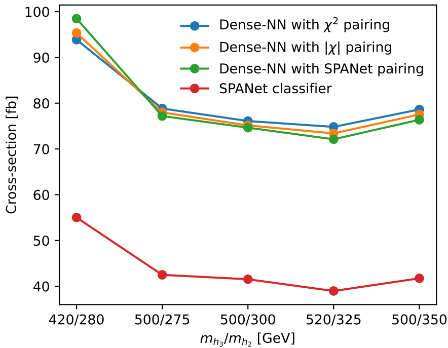
95% CL limit on \sigma(pp \rightarrow hhh)
