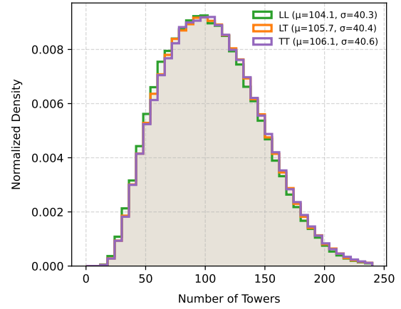
(b) Number of calorimeter towers
