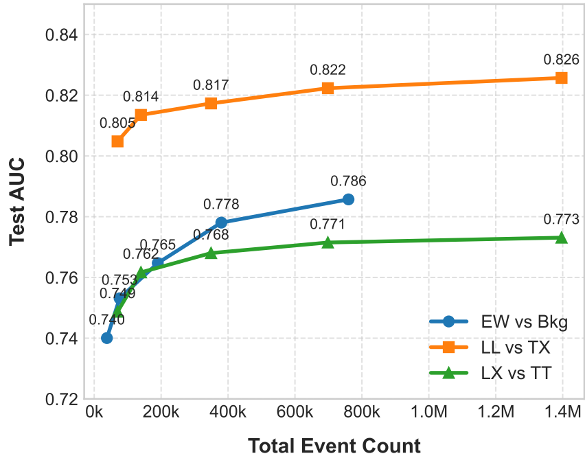
Figure 14: Test AUC performance as a function of total event count for the three classification tasks evaluated using the High-Level ParT model.
