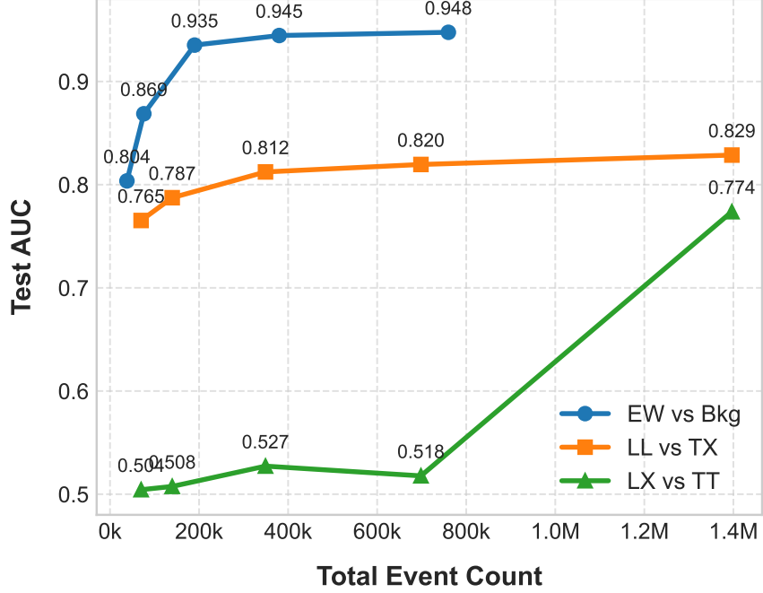
Figure 15: Test AUC performance as a function of total event count for the three classification tasks evaluated using the Low-Level ParT model.
