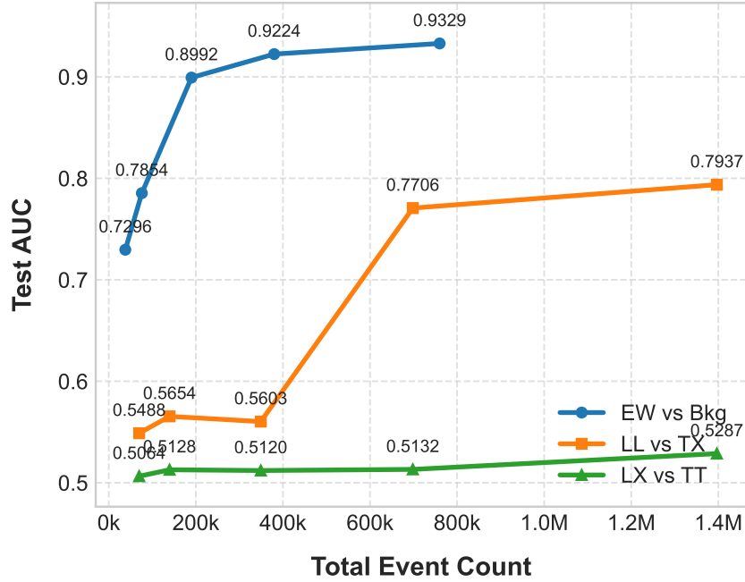
Figure 15: Test AUC performance as a function of total event count for the three classification tasks evaluated on Fold 0 using the Low-Level EFlow ParT model.
