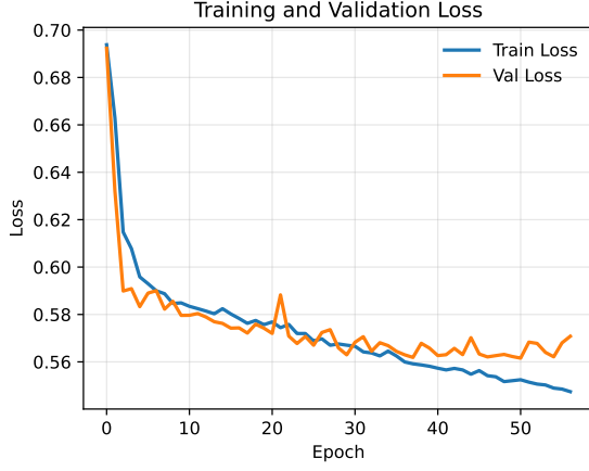
(a) Loss (High-Level features)
