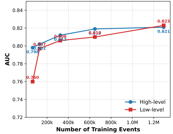
(b) LL vs. TX
