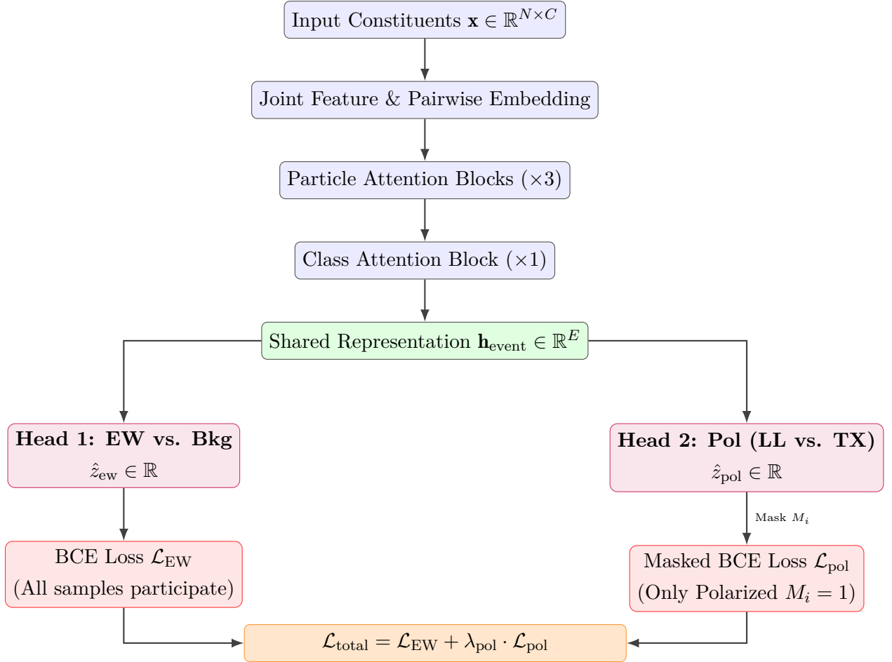
Figure 16: Architecture of the Multi-Head Particle Transformer with shared attention backbone and dual heads governed by masked multi-task loss.
