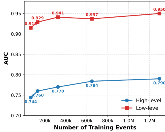
(a) EW vs. Bkg.
