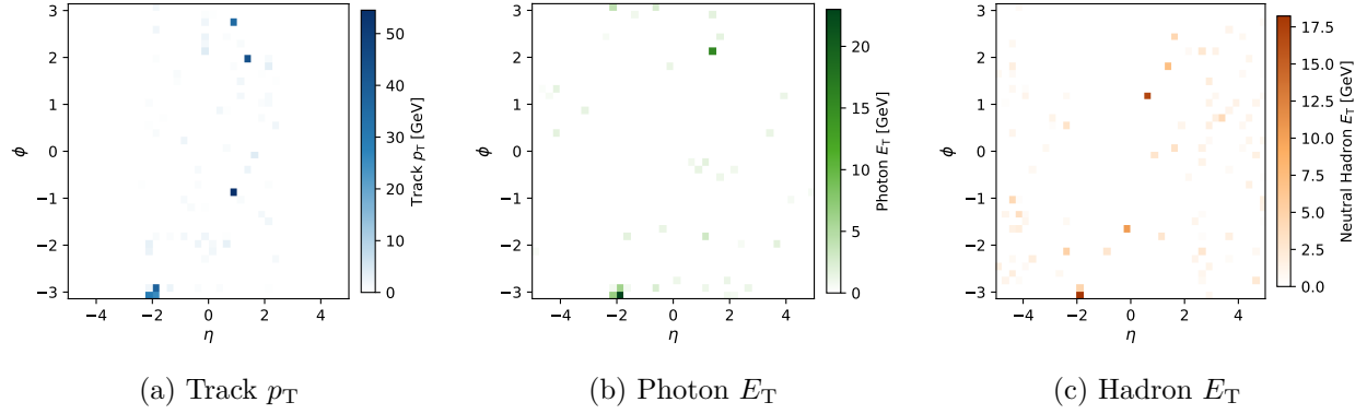
Figure 18: Single-event calorimeter and tracker image representations for a EW W^+W^+jj event on a 40 \times 40 grid ( \eta \in [-5, 5] , \phi \in [-\pi, \pi] ).
