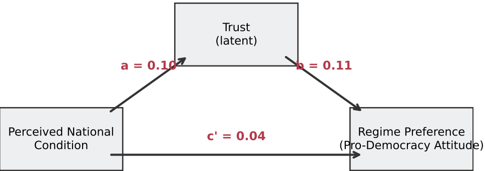
Path model -- Nepal-only, Wave 2013
