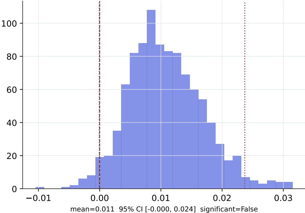
Bootstrapped indirect effect ( a \times b ), n=1000
