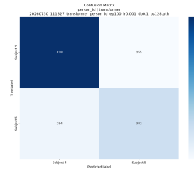
(c) Transformer (Person ID)
