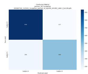
(b) Inception (Person ID)
