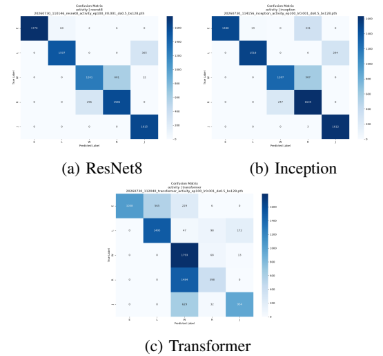
Fig. 8: Confusion Matrices for Activity Recognition.
