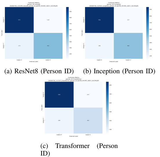
Fig. 9: Confusion Matrices for Person Identification.
