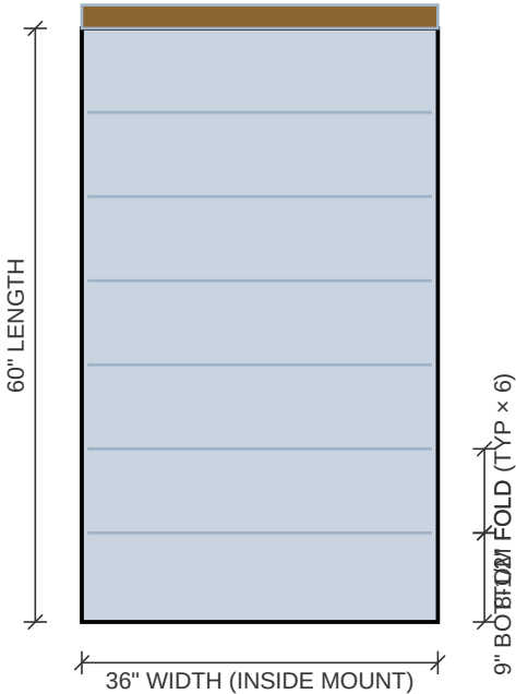
FRONT ELEVATION — FLAT ROMAN
