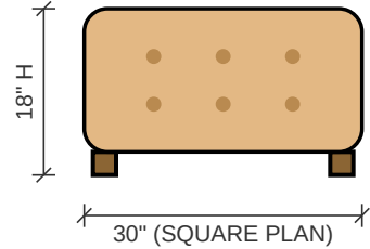
OTTOMAN — FRONT ELEVATION
