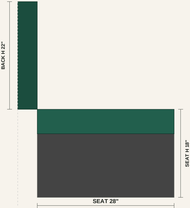
SIDE SECTION
