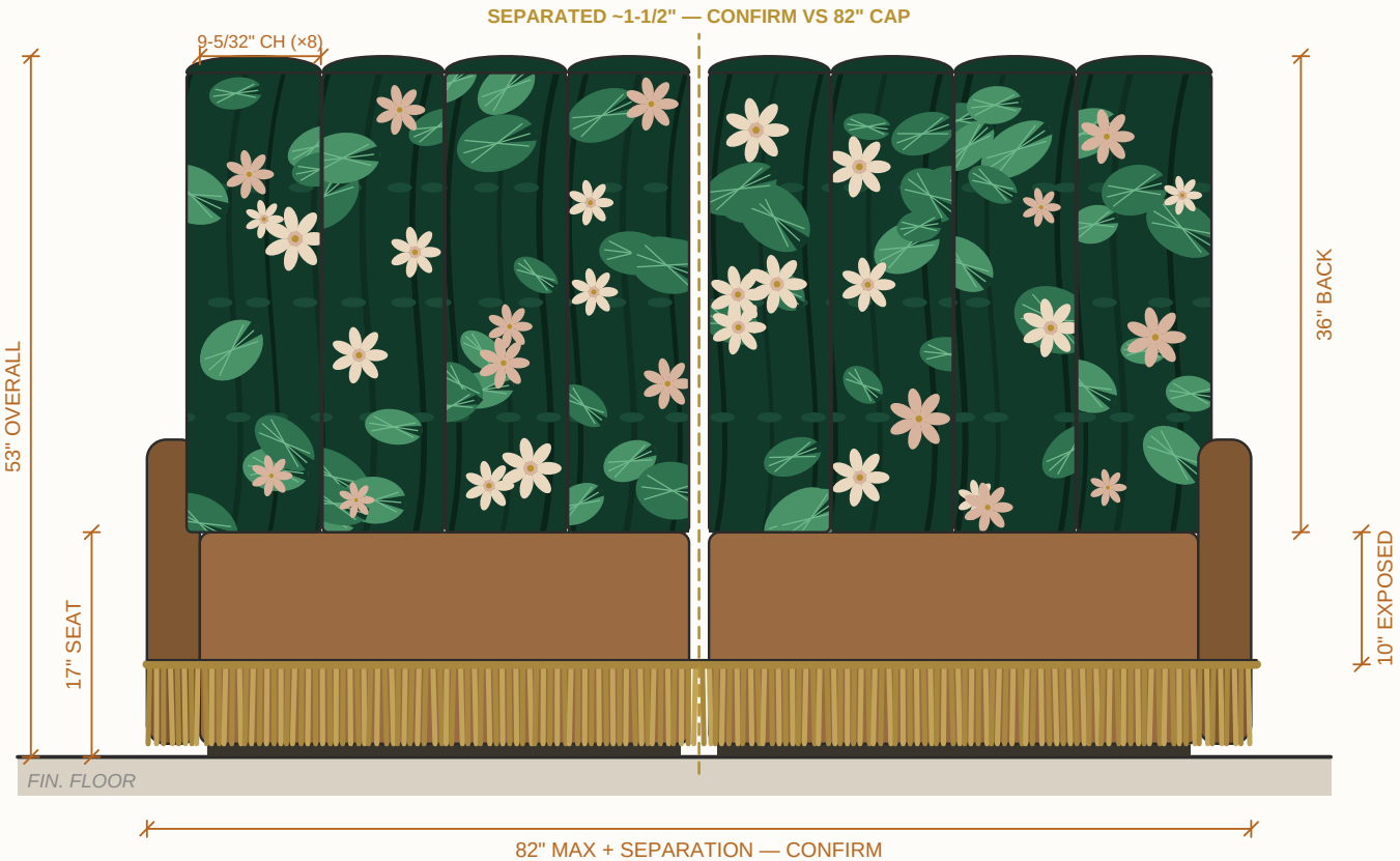
FRONT ELEVATION (DEVELOPED)
