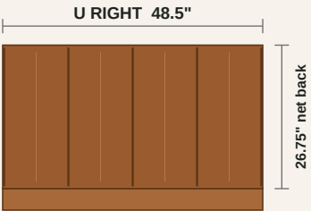
4 x 12" channels + 0.25" end trim each side seat cushion: plain cognac (height shown nominal)
