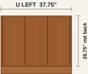
3 x 12" channels + 0.875" end trim each side seat cushion: plain cognac (height shown nominal)
