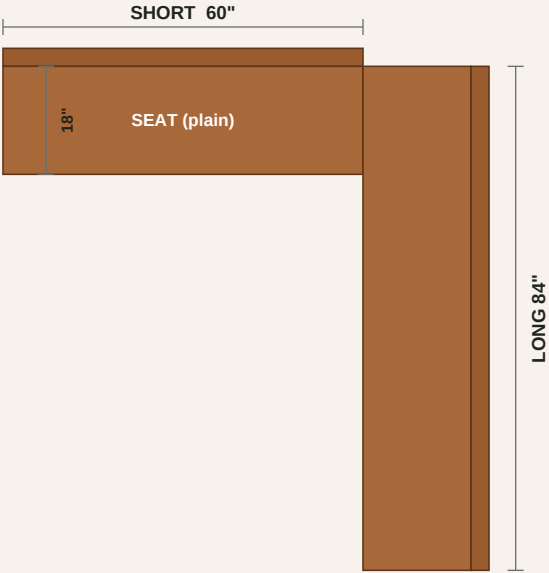
L-SHAPED CORNER BANQUETTE — PLAN
