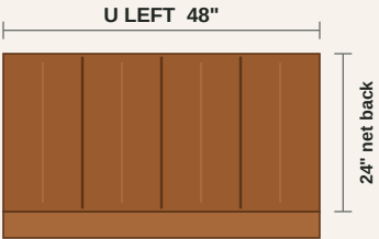
4 x 12" channels seat cushion: plain cognac (height shown nominal)
