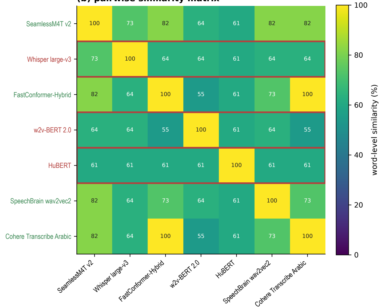
(b) pairwise similarity matrix
