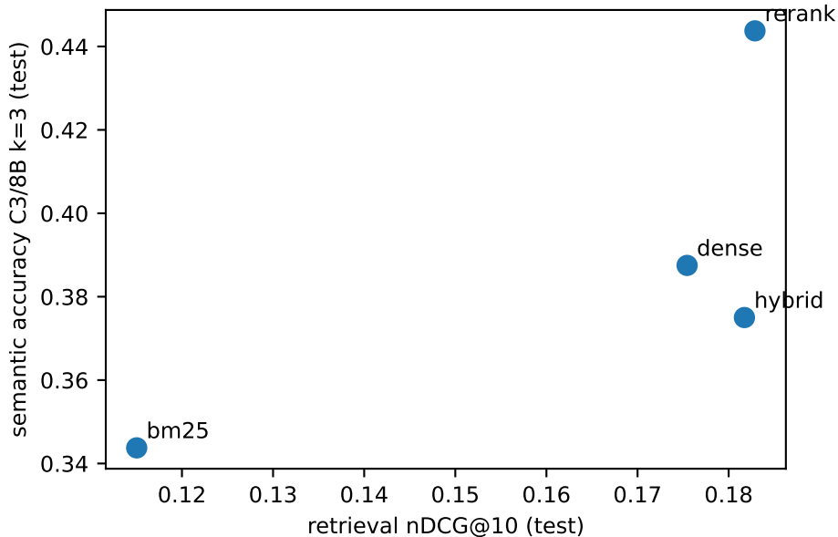
Retrieval -> semantic transfer (frozen)
