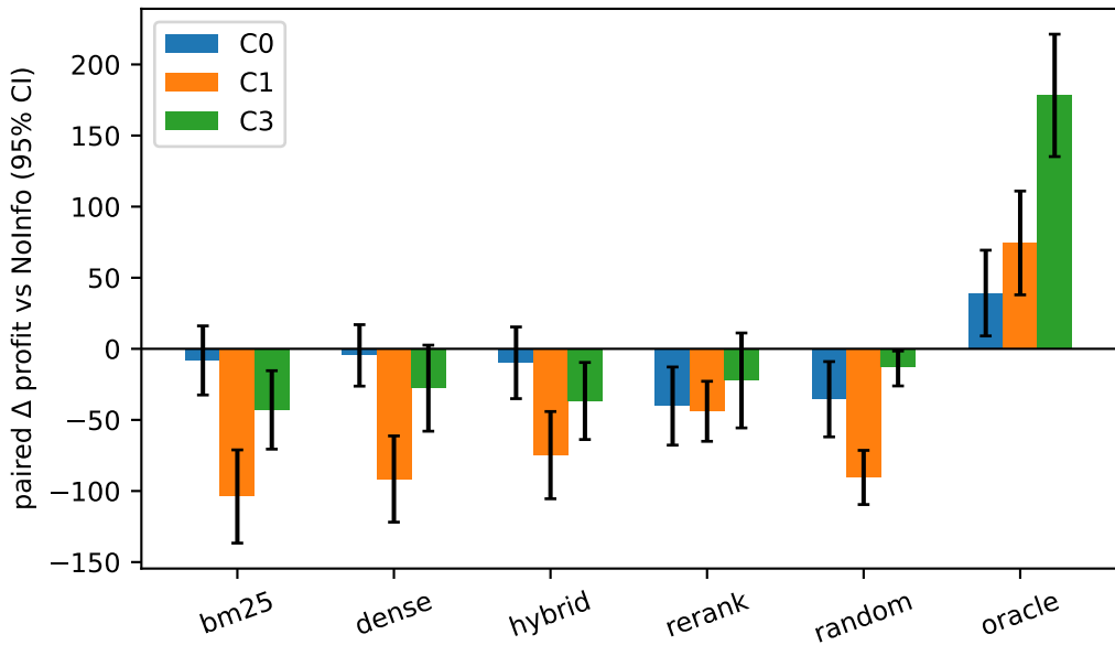
Retriever x Consumer utility (8B, k=3)
