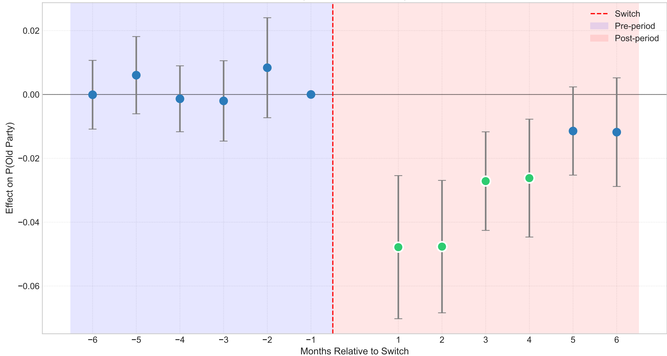
Figure 1: Event Study - Linguistic Adaptation After Party Switching (Pre-trends p = 0.789)
