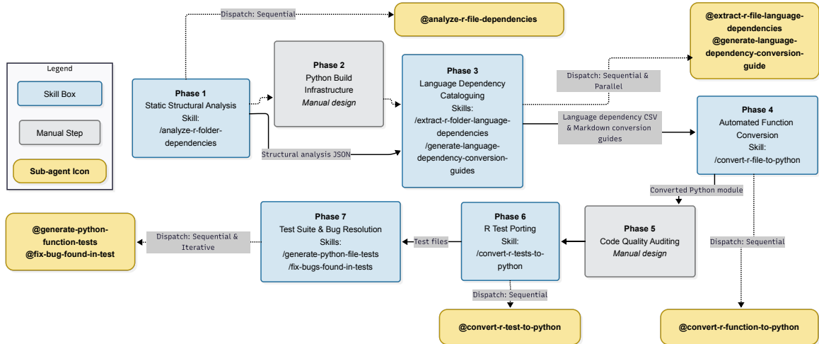
Figure 1: Overview of the seven-phase AI-assisted R-to-Python conversion methodology. The pipeline proceeds from static structural analysis (Phase 1) through build infrastructure (Phase 2), language dependency cataloguing (Phase 3), automated function conversion and assembly (Phase 4), code quality auditing (Phase 5), R test porting (Phase 6), and comprehensive test-suite construction with iterative bug resolution (Phase 7). The phase outputs form a directed chain of artefacts consumed by subsequent phases. Skills (top-level slash commands) and their sub-agents are indicated for each phase; the dispatch mode (sequential, parallel, or iterative) of each sub-agent fleet is shown explicitly.
