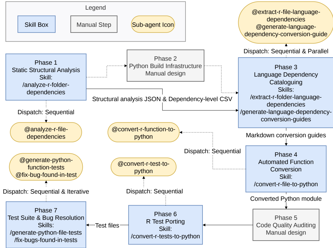
Figure 1: Overview of the seven-phase AI-assisted R-to-Python conversion methodology. The pipeline proceeds from static structural analysis (Phase 1) through build infrastructure (Phase 2), language dependency cataloguing (Phase 3), automated function conversion and assembly (Phase 4), code quality auditing (Phase 5), R test porting (Phase 6), and comprehensive test-suite construction with iterative bug resolution (Phase 7). The phase outputs form a directed chain of artefacts consumed by subsequent phases. Skills (top-level slash commands) and their sub-agents are indicated for each phase; the dispatch mode (sequential, parallel, or iterative) of each sub-agent fleet is shown explicitly.
