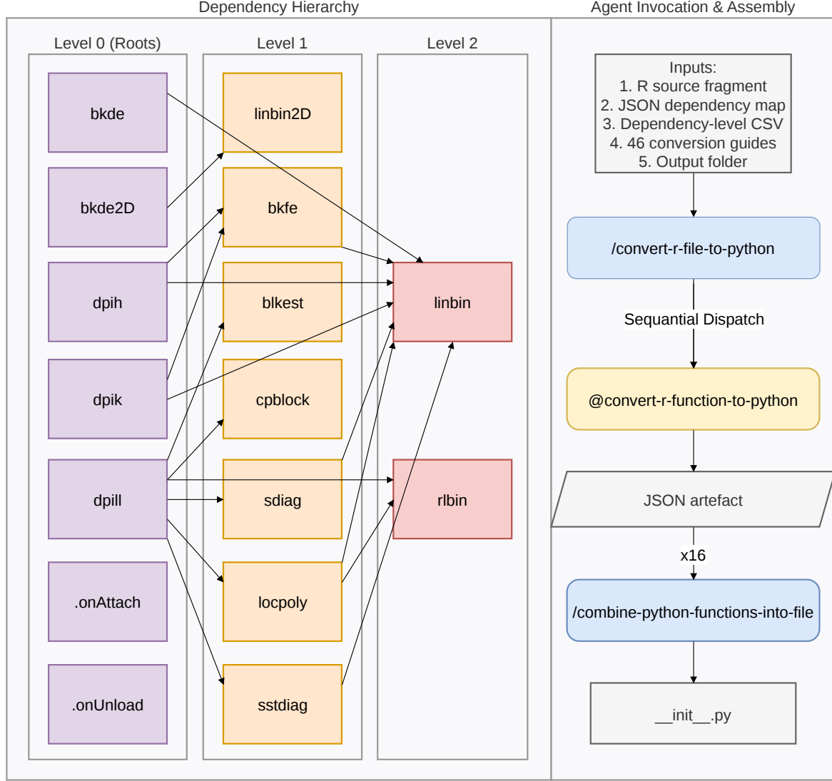
Figure 5: Phase 4: topologically ordered function conversion and package assembly. Functions are converted in leaf-to-root order so that each conversion agent can inspect the Python calling convention of already-converted internal dependencies. The /convert-r-file-to-python skill derives the conversion order from the dependency-level CSV produced in Phase 1 and dispatches the @convert-r-function-to-python sub-agent sequentially. The /combine-python-functions-into-file skill then assembles the 16 resulting JSON artefacts into the final __init__.py , correcting import paths and deduplicating imports.
