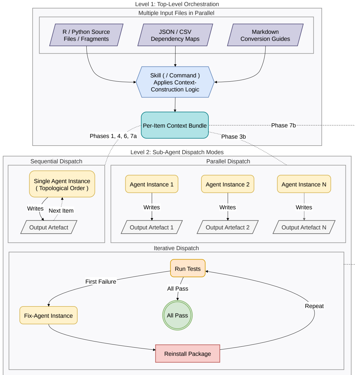
Figure 2: Skill-agent orchestration architecture. A skill (slash command) acts as an orchestrator: it assembles per-item context bundles from shared inputs and dispatches sub-agents in one of three modes. Sequential dispatch (Phases 1, 4, 6, and 7a) is used when each agent invocation must have access to the outputs of prior invocations. Parallel dispatch (Phase 3b) is used when agent invocations are independent and latency is the binding constraint. Iterative dispatch (Phase 7b) repeatedly invokes a fix-agent until a stopping criterion (all tests pass) is met.
