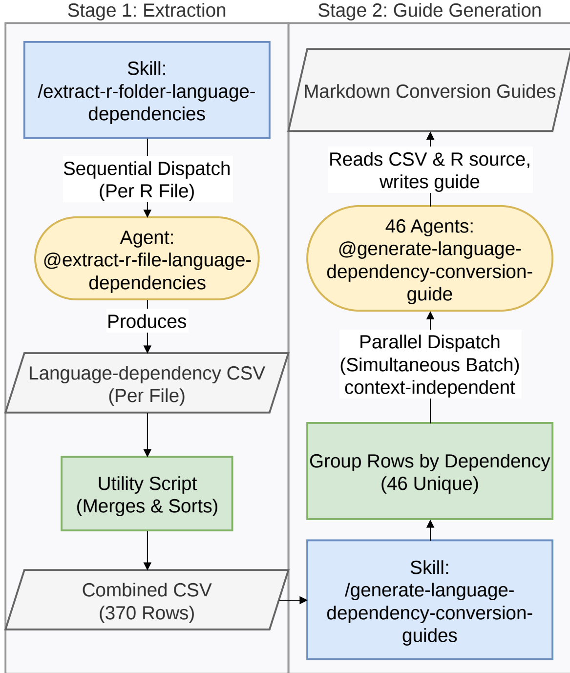
Figure 4: Phase 3: language dependency extraction and parallel conversion guide generation. The first stage extracts the complete call-site table (370 rows, 4 columns) from the R source via sequential agent dispatch. The second stage launches 46 sub-agent instances simultaneously—one per unique language dependency—each producing a Markdown guide specifying the exact Python translation strategy with code examples. Parallel dispatch is appropriate because the guide for each dependency is context-independent of all other guides.
