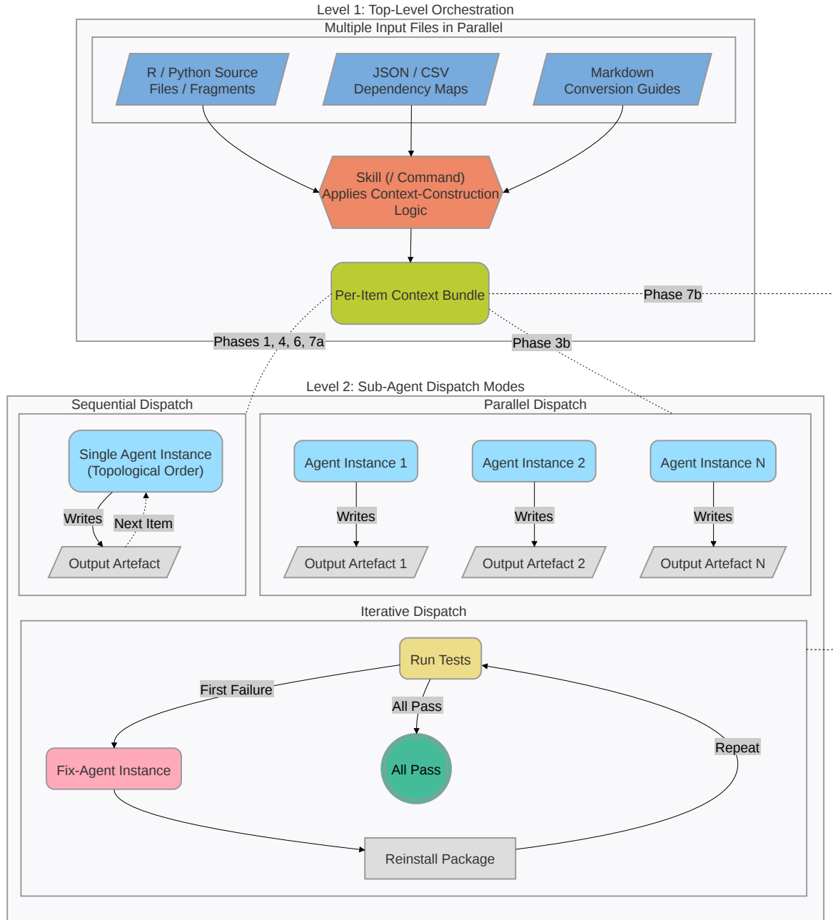
Figure 2: Skill-agent orchestration architecture. A skill (slash command) acts as an orchestrator: it assembles per-item context bundles from shared inputs and dispatches sub-agents in one of three modes. Sequential dispatch (Phases 1, 4, 6, and 7a) is used when each agent invocation must have access to the outputs of prior invocations. Parallel dispatch (Phase 3b) is used when agent invocations are independent and latency is the binding constraint. Iterative dispatch (Phase 7b) repeatedly invokes a fix-agent until a stopping criterion (all tests pass) is met.
