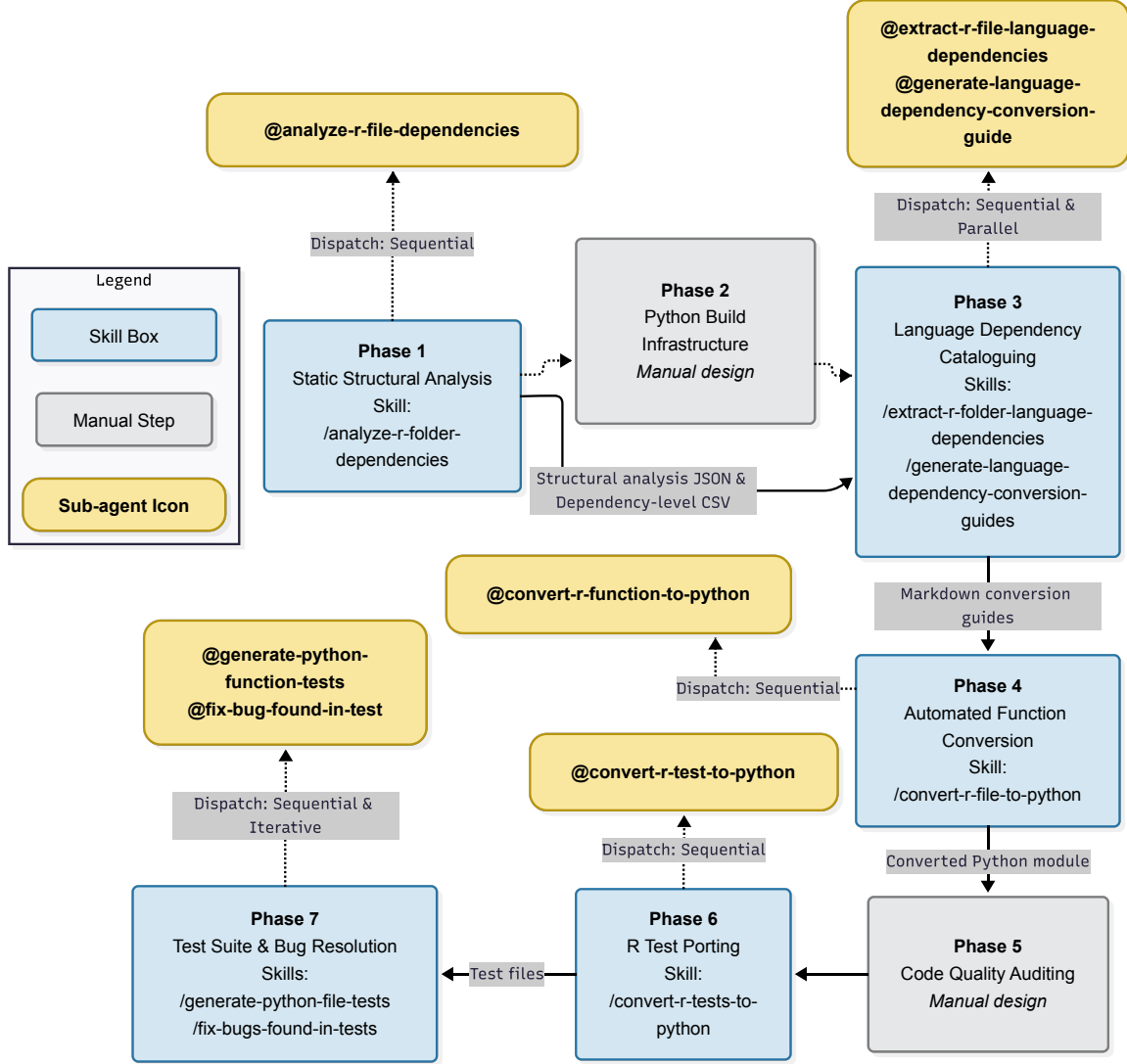
Figure 1: Overview of the seven-phase AI-assisted R-to-Python conversion methodology. The pipeline proceeds from static structural analysis (Phase 1) through build infrastructure (Phase 2), language dependency cataloguing (Phase 3), automated function conversion and assembly (Phase 4), code quality auditing (Phase 5), R test porting (Phase 6), and comprehensive test-suite construction with iterative bug resolution (Phase 7). The phase outputs form a directed chain of artefacts consumed by subsequent phases. Skills (top-level slash commands) and their sub-agents are indicated for each phase; the dispatch mode (sequential, parallel, or iterative) of each sub-agent fleet is shown explicitly.
