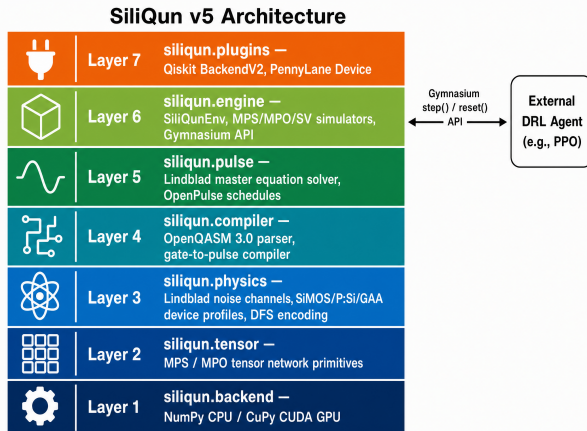
Fig. 5. SiliQun architecture. The simulator is organised into seven layers: the Gymnasium RL environment ( silique.engine ), the Lindblad pulse solver ( silique.pulse ), the OpenQASM 3.0 compiler ( silique.compiler ), the physics layer with device profiles and noise channels ( silique.physics ), third-party framework plugins ( silique.plugins ), the numerical backend ( silique.backend ), and the tensor-network primitives ( silique.tensor ). An external DRL agent (e.g., PPO) interacts with SiliQun exclusively through the standard Gymnasium step/reset API.
