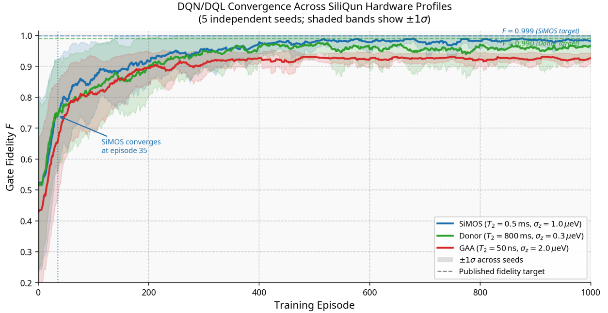
Fig. 5. Learning curves for the DQN/DQL agent on all three SiliQun hardware profiles (5 independent seeds each; shaded bands show \pm 1\sigma ). Dashed lines mark the published fidelity targets: F > 0.999 for SiMOS [29] and F > 0.990 for donor [30]. No published baseline exists for GAA. All three agents converge from a near-random initial policy to a stable high-fidelity regime within 200–400 episodes, with narrow confidence bands confirming cross-seed reproducibility.
