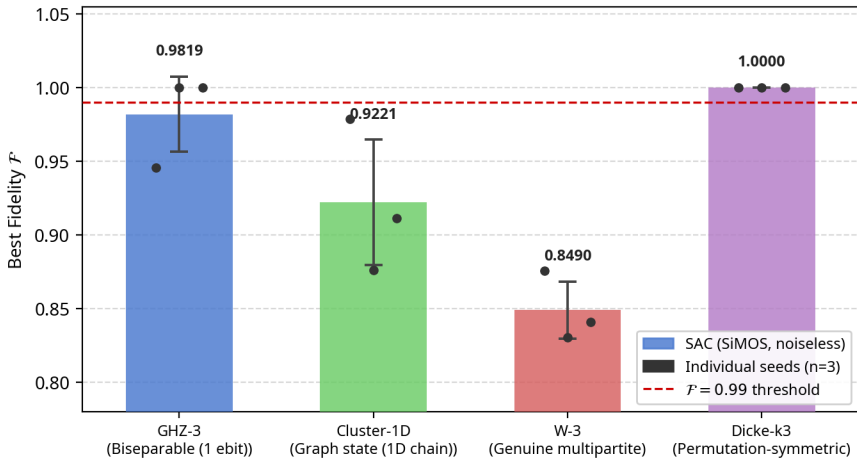
Extension 4: SAC Generalisation Across Entanglement Classes (SiMOS device, 3-qubit targets, 3 seeds each)
