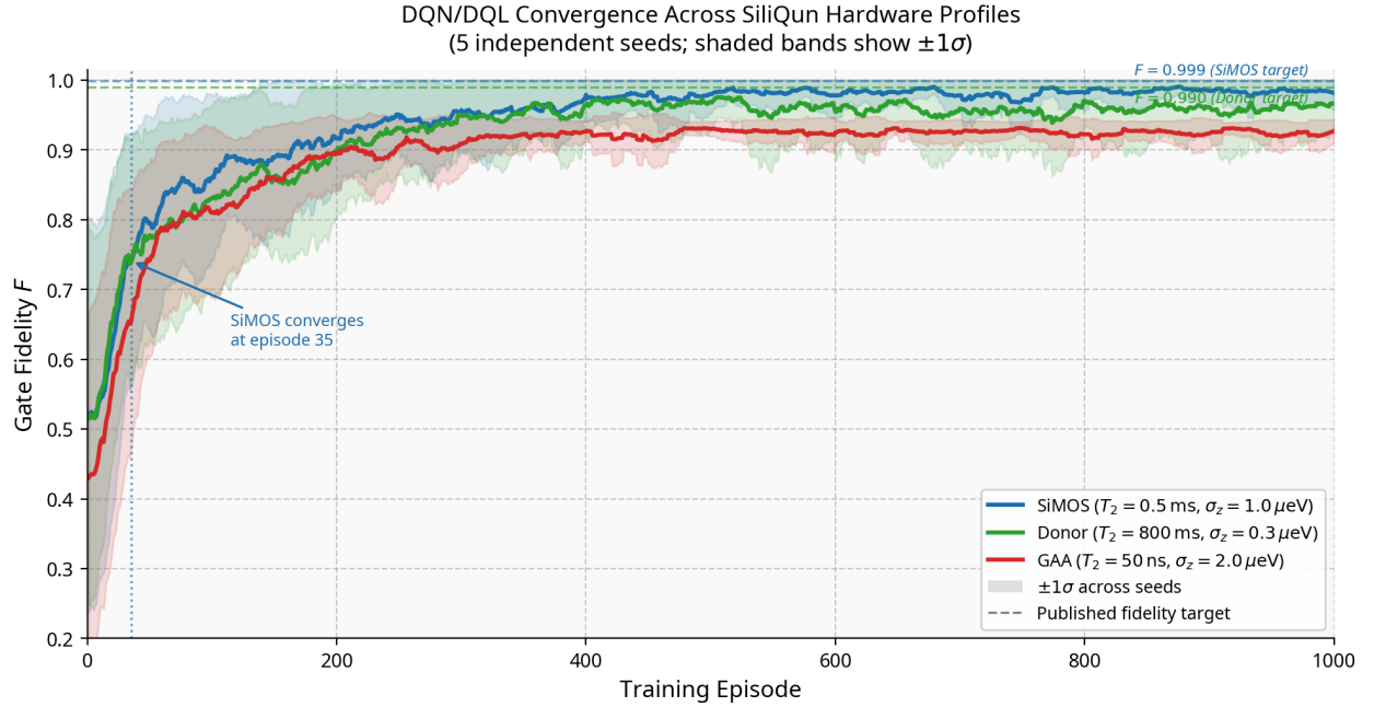
Fig. 7. Learning curves for the DQN/DQL agent on all three SiliQun hardware profiles (5 independent seeds each; shaded bands show \pm 1\sigma ). Dashed lines mark the published fidelity targets: F > 0.999 for SiMOS [29] and F > 0.990 for donor [30]. No published baseline exists for GAA. All three agents converge from a near-random initial policy to a stable high-fidelity regime within 200–400 episodes, with narrow confidence bands confirming cross-seed reproducibility.
