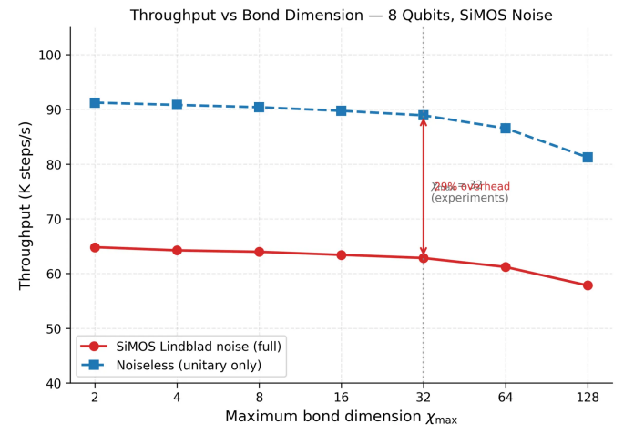
Fig. 4. Throughput versus maximum bond dimension \chi_{\text{max}} for an 8-qubit register under SiMOS Lindblad noise. The noiseless MPS throughput (dashed blue) decreases by only 11% as \chi_{\text{max}} increases from 2 to 128, confirming sub-quadratic scaling. Under full SiMOS noise (solid red), throughput decreases by 29% relative to the noiseless baseline at \chi_{\text{max}} = 32 (the value used in all experiments), consistent with the mean noise overhead of 27.7%. The vertical dotted line marks the experimental value \chi_{\text{max}} = 32 .
