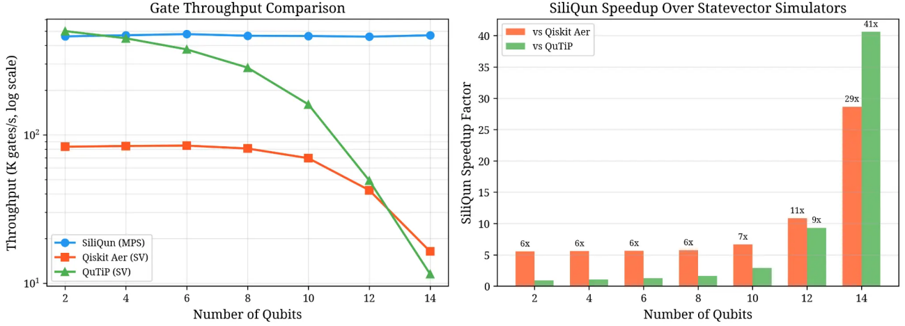
Fig. 9. Gate throughput comparison and SiliQun speedup factor. Left: Throughput (K gates/s, log scale) for SiliQun MPS (blue), Qiskit Aer statevector (orange), and QuTiP statevector (green) as a function of qubit count. SiliQun maintains near-constant throughput across all qubit counts due to MPS compression; statevector simulators exhibit exponential degradation. Right: SiliQun speedup factor relative to Qiskit Aer and QuTiP. At 14 qubits, SiliQun is 29 \times faster than Qiskit Aer and 41 \times faster than QuTiP, confirming the scalability advantage of the MPS backend for DRL training workloads.
