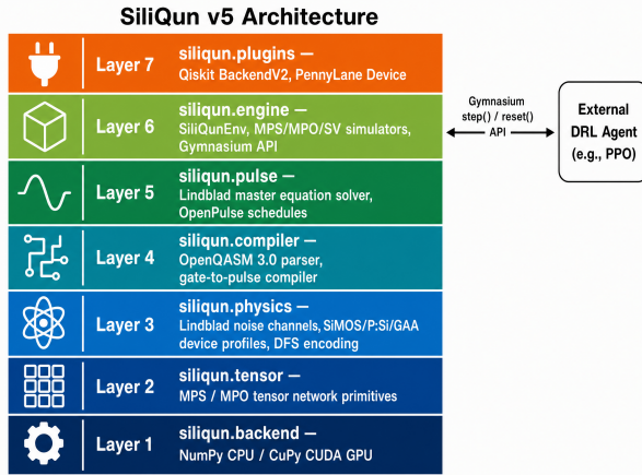
Fig. 5. SiliQun architecture. The simulator is organised into seven layers: the Gymnasium RL environment ( siliqun.engine ), the Lindblad pulse solver ( siliqun.pulse ), the OpenQASM 3.0 compiler ( siliqun.compiler ), the physics layer with device profiles and noise channels ( siliqun.physics ), third-party framework plugins ( siliqun.plugins ), the numerical backend ( siliqun.backend ), and the tensor-network primitives ( siliqun.tensor ). An external DRL agent (e.g., PPO) interacts with SiliQun exclusively through the standard Gymnasium step/reset API.
