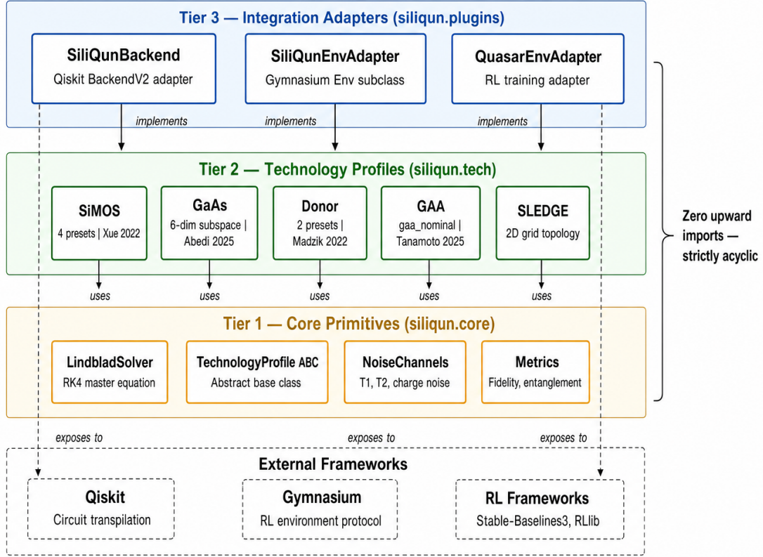
Fig. 3. The SiliQun three-tier package architecture. Tier 1 ( siliqun.core ) provides hardware-agnostic simulation primitives including the Lindblad solver, abstract base classes, and quantum information metrics. Tier 2 ( siliqun.tech ) implements five technology-specific physics modules (SiMOS, GaAs, Donor, GAA, SLEDGE), each grounded in published calibration data. Tier 3 ( siliqun.plugins ) exposes the physics engine through three integration adapters: a Qiskit BackendV2 ( SiliQunBackend ), a Gymnasium Env ( SiliQunEnvAdapter ), and an extended RL training adapter ( SiliQunRLAdapter ). Dependency arrows are strictly downward; Tier 1 has zero imports from Tier 2 or Tier 3.
