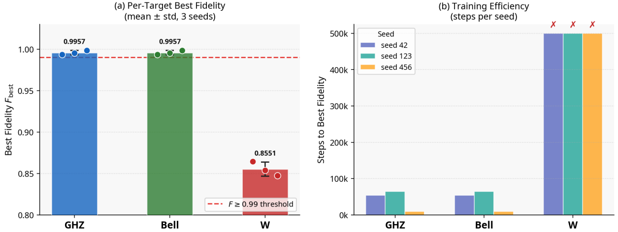
Fig. 10. Extension 4 results summary. (a) Mean best fidelity \bar{F}_{\text{best}} per target state (bars: mean; error bars: \pm\sigma ; dots: individual seed values). The dashed red line marks the F \geq 0.99 threshold. GHZ-3 and Bell-3 exceed the threshold across all three seeds; W-3 plateaus at \bar{F} = 0.8551 , below the threshold. (b) Steps to best fidelity per seed. Seed 456 converges in 9,209 steps for GHZ/Bell, roughly 6\times faster than seeds 42 and 123. W-state runs exhaust the full 5 \times 10^5 step budget (marked \times ). Hardware: RTX 2070 Max-Q 8 GB VRAM.
