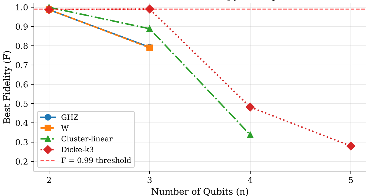
QUASAR v11 Baseline: Fidelity vs Qubit Count (Without DEHB Entropy Tuning)
