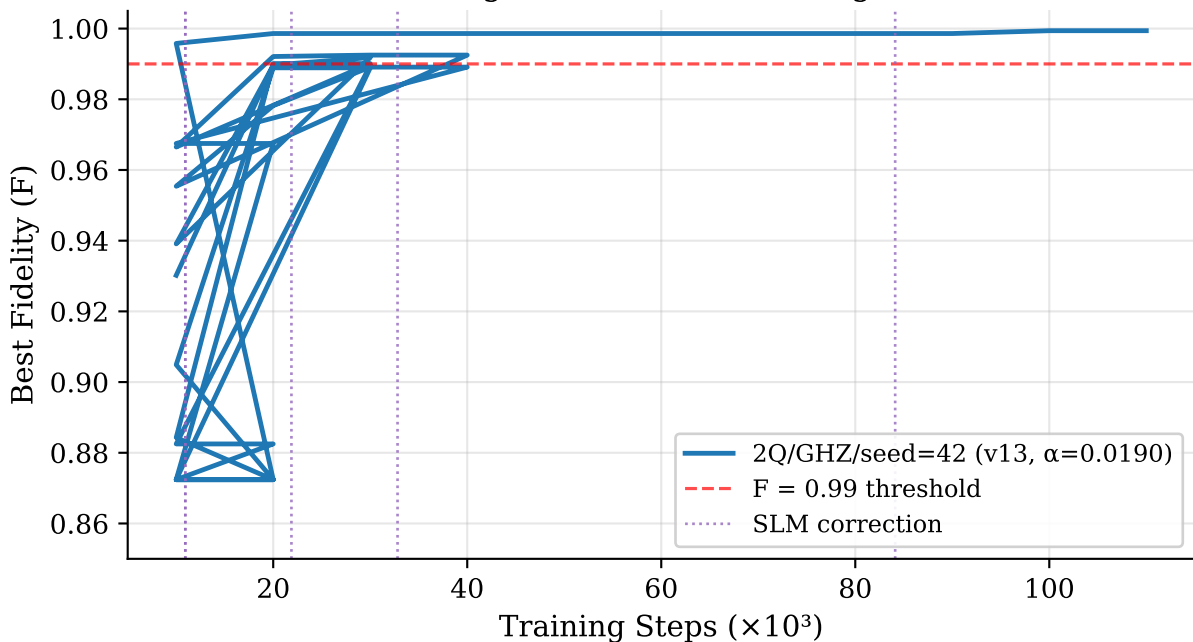
QUASAR v13: Fidelity vs Training Steps (GHZ Target, 2 Qubits, Full-Budget Run)
