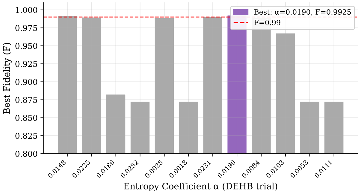
DEHB Hyperparameter Search: \alpha vs Best Fidelity (GHZ Target, 2 Qubits)
